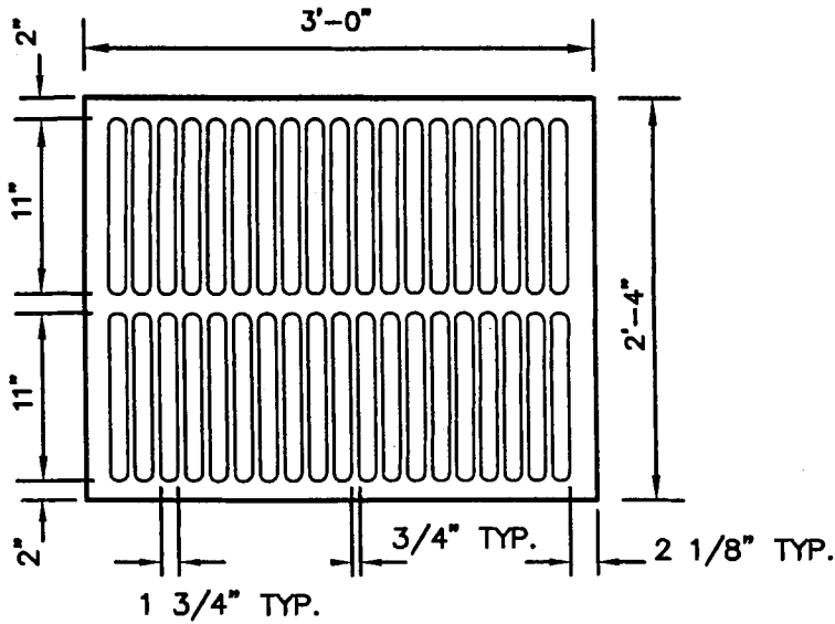
CAST IRON GRATE INDEX SHT. 232
